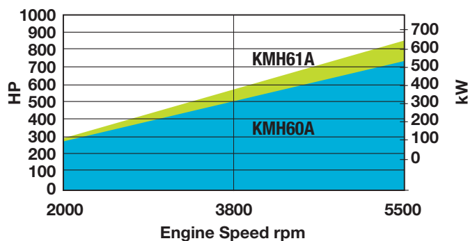
Power Diagram for Pleasure Use
