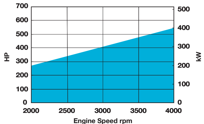
Power Diagram for Pleasure Use
